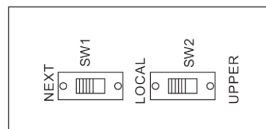
Uplink unit
